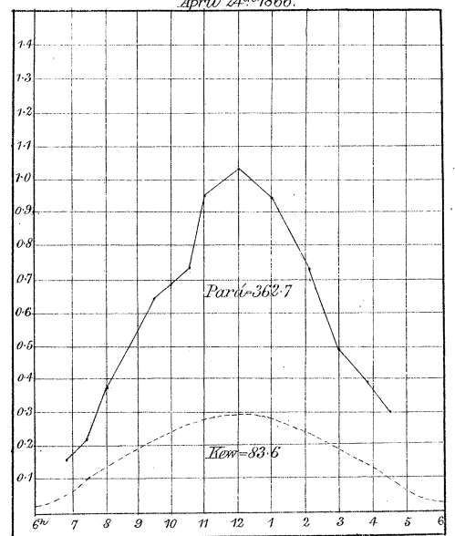
Fig. 14. Curve showing March of Total Chemical Intensity for Sunshine. Pará, April 1866.
